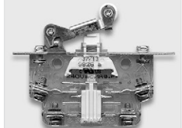
S826 a / S926 a Roller lever, mounting brackets, silver contacts and M3 screws with saddle clamp
